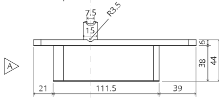
Vista frontal
