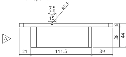
Vista frontal
